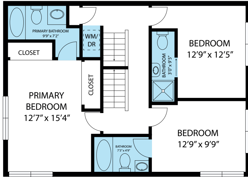
3RD FLOOR
